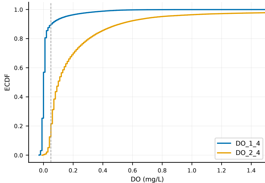
Value distribution (ECDF)
